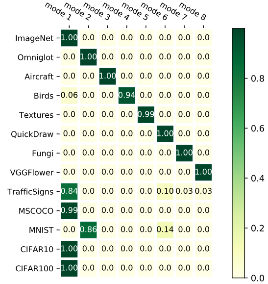
Figure 3. Selection gates of the domain-specific parameter set.
